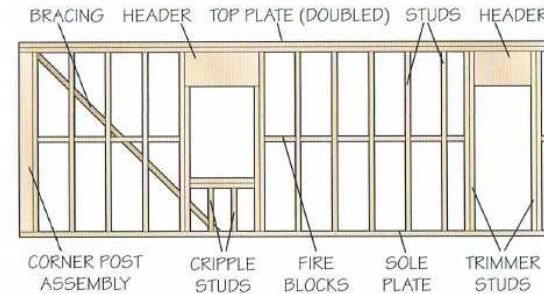
Wall frame
