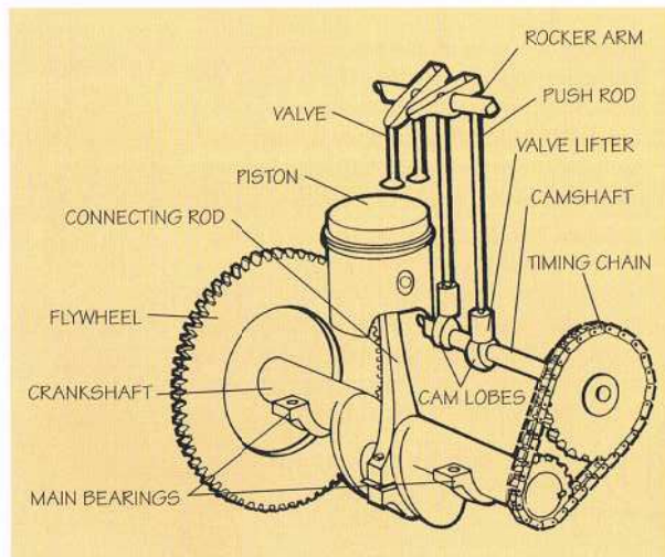
Engine valve train and flywheel
