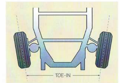
Front wheel toe alignment viewed from top of car
