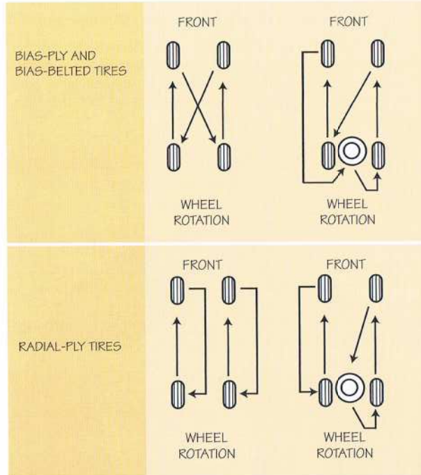
Radial-ply and bias-ply or bias-belted tires have different rotation patterns.
