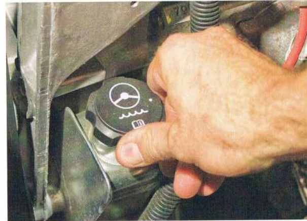
Checking the power steering fluid indicator and add power steering fluid if it shows "low."
