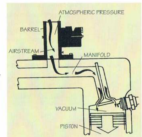
Higher atmospheric pressure makes air flow into the engine. The intake stroke creates a vacuum (low pressure).
