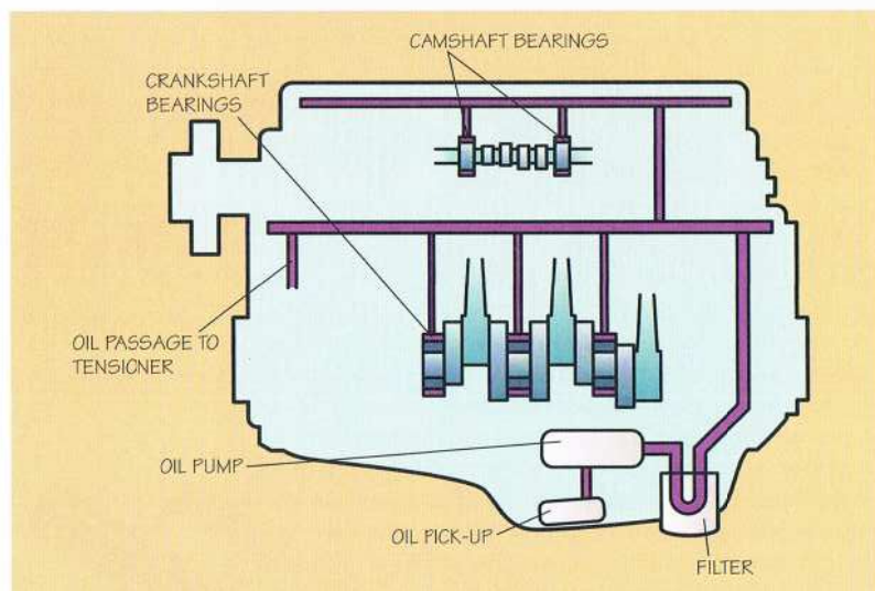
Lubrication system components
