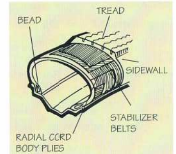
Most passenger car tires use the radial-ply design.
