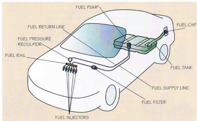
Typical fuel injection system
