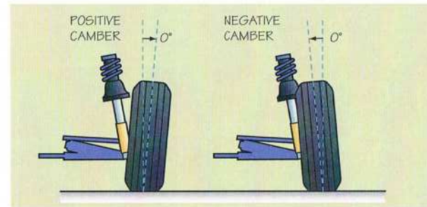
A front wheel, viewed from the front of the car
