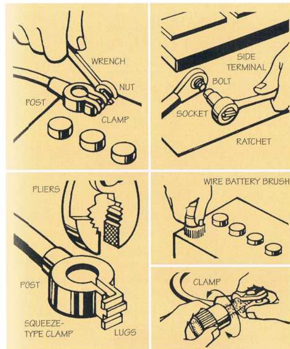
Battery connections must be clean and tight.
