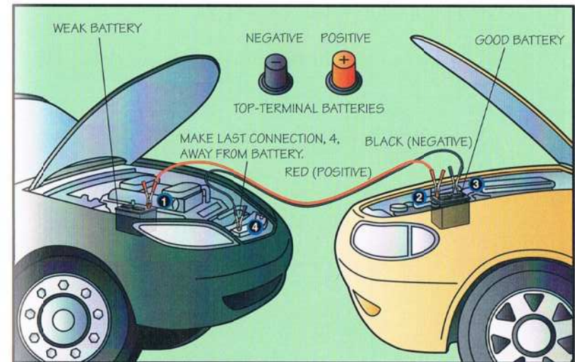
Correct jumper cable connections
