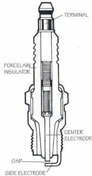
Spark plug construction
