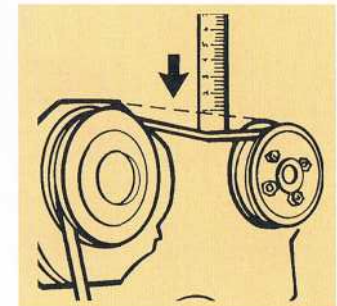
Checking drive belt tension
