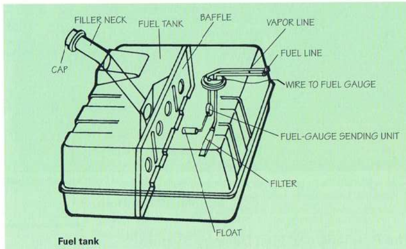
Fuel tank
