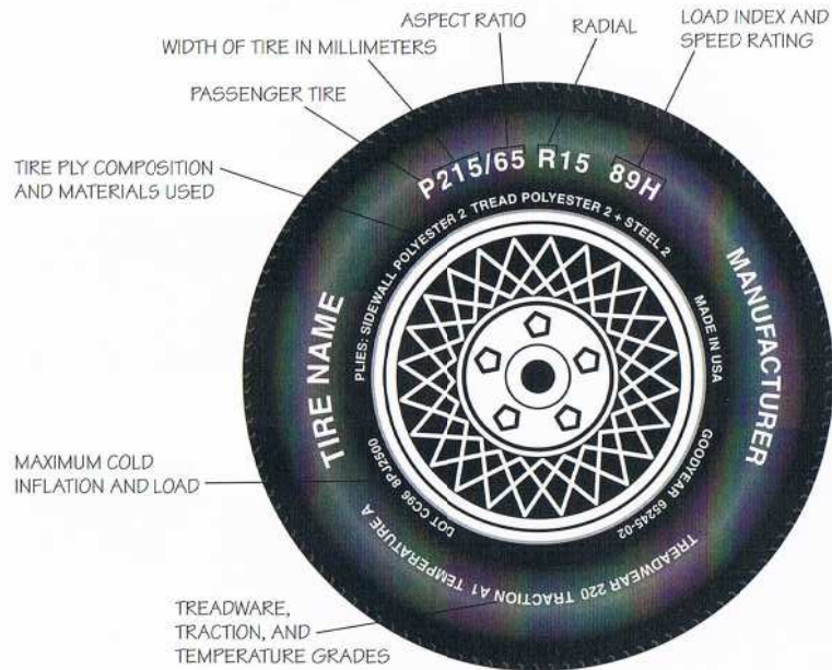
Tire specifications are on the sidewall.
