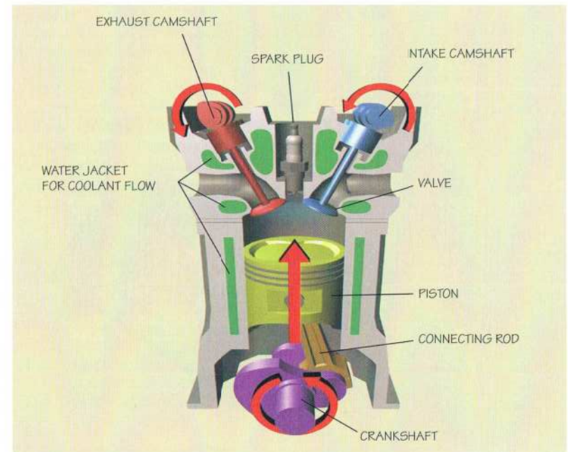
Combustion chamber components
