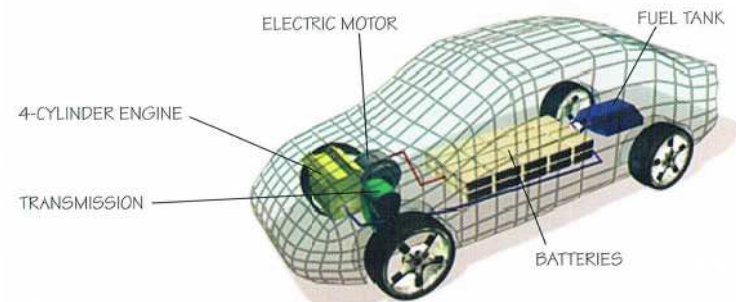
Gasoline-electric parallel hybrid drive train
