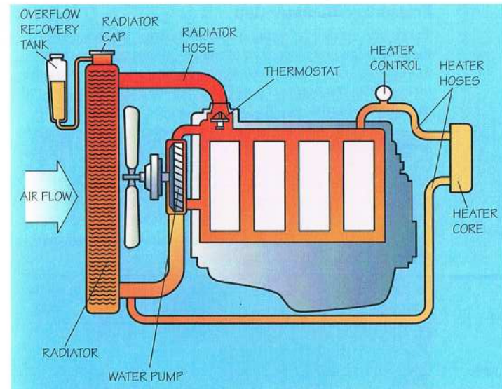
Cooling system components
