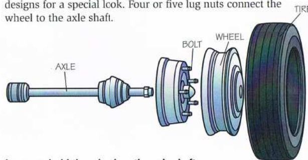
Lug nuts hold the wheel on the axle shaft.
